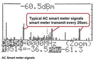
AC Smart meter signals
