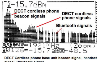
DECT Cordless phone base unit beacon signal, handset signal, Bluetooth signal
