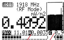
Duty Cycle for digital RF burst signals unit is xx.x% All Average value is peak value x Duty cycle
